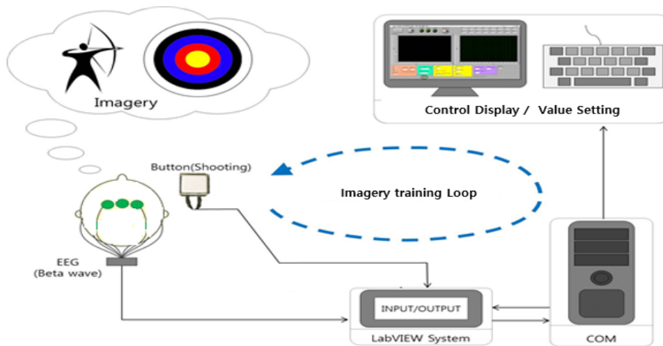
Figure 3. The structure and flow of the Labview program
