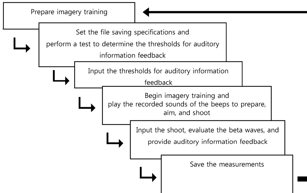
Figure 2. The structure and flow of the Labview program
