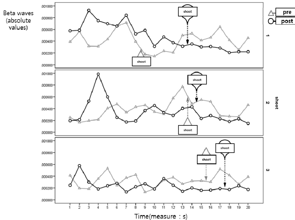
Figure 4. Changes in beta waves over 20 seconds before and after a shoot, across all archers
